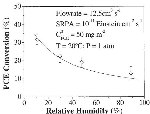
Figure 8. PCE conversion for different relative humidity values.
